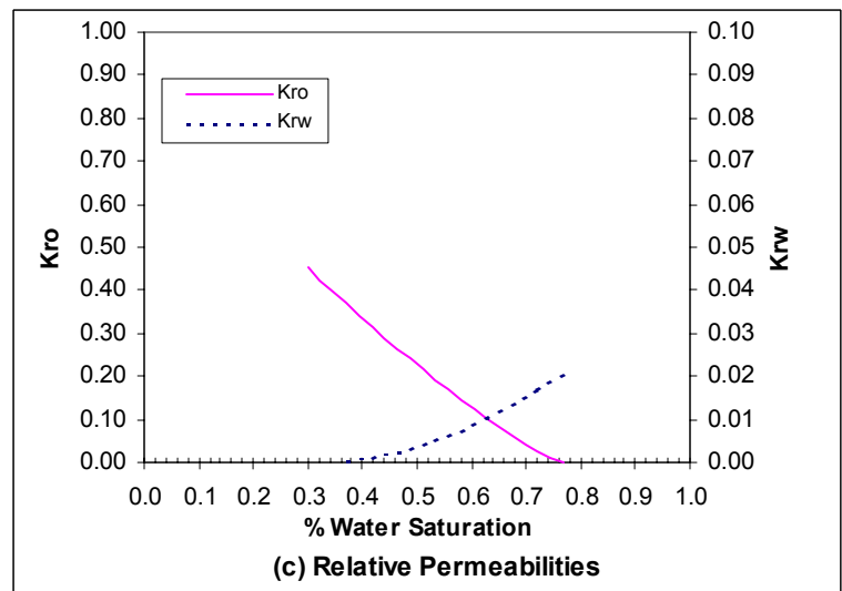
Figure A18: Coreflood Simulator Results for Waterflood of Yates Crude Oil in Berea Core with Anionic Surfactant Concentration of 1500 ppm
