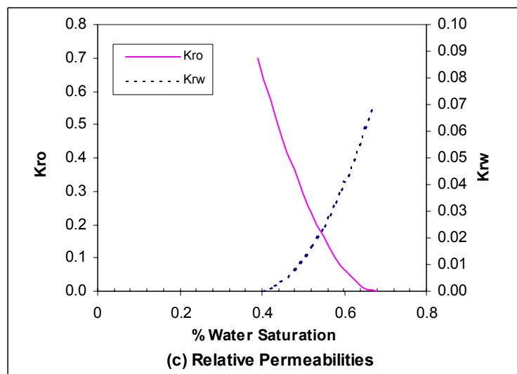
Figure A1: Coreflood Simulator Results for Waterflood of Decane in Berea Core with Nonionic Surfactant Concentration of 0 ppm
