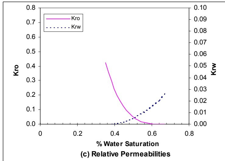
Figure A3: Coreflood Simulator Results for Waterflood of Decane in Berea Core with Nonionic Surfactant Concentration of 1500 ppm
