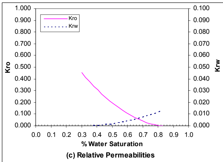
Figure A19: Coreflood Simulator Results for Waterflood of Yates Crude Oil in Berea Core with Anionic Surfactant Concentration of 3500 ppm
