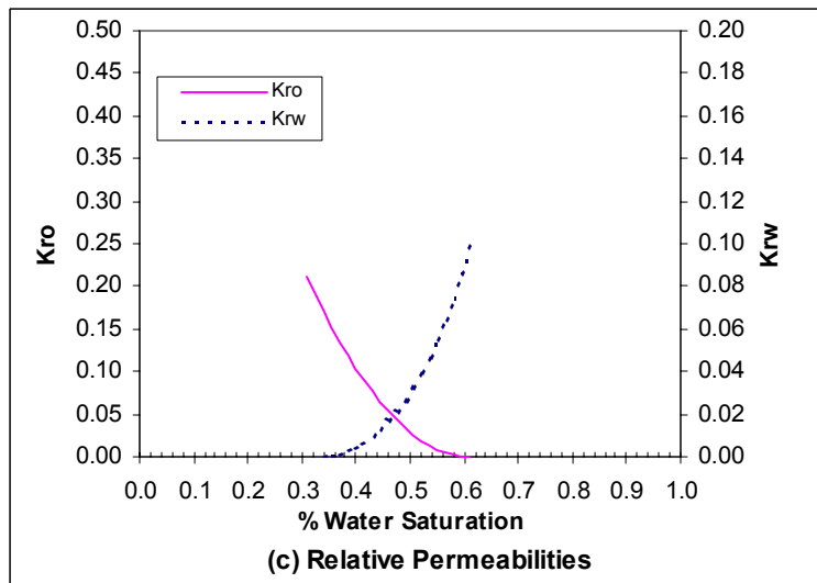
Figure A13: Coreflood Simulator Results for Waterflood of Decane in Berea Core with Anionic Surfactant Concentration of 1500 ppm
