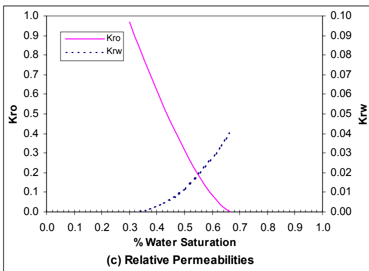
Figure A16: Coreflood Simulator Results for Waterflood of Yates Crude Oil in Berea Core with Anionic Surfactant Concentration of 0 ppm
