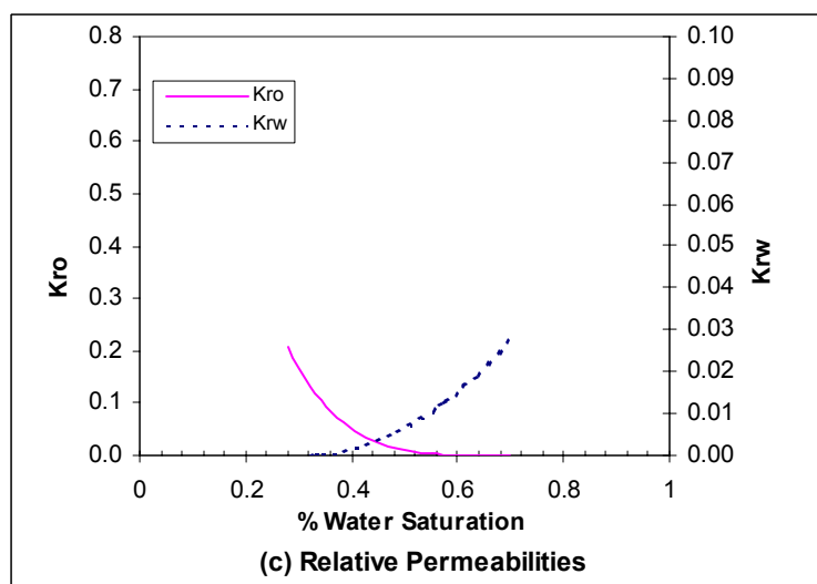
Figure A5: Coreflood Simulator Results for Waterflood of Decane in Berea Core with Nonionic Surfactant Concentration of 5000 ppm
