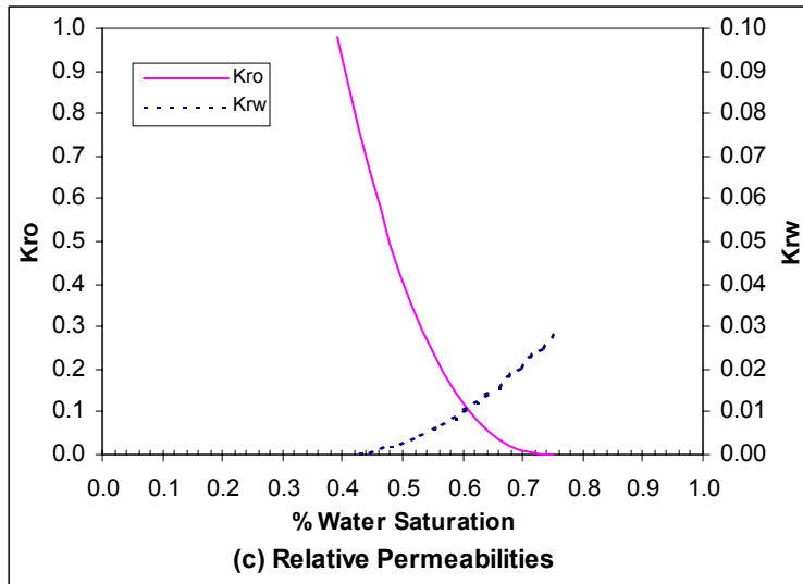
Figure A6: Coreflood Simulator Results for Waterflood of Yates Crude Oil in Berea Core with Nonionic Surfactant Concentration of 0 ppm
