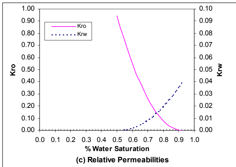
Figure A8: Coreflood Simulator Results for Waterflood of Yates Crude Oil in Berea Core with Nonionic Surfactant Concentration of 1500 ppm
