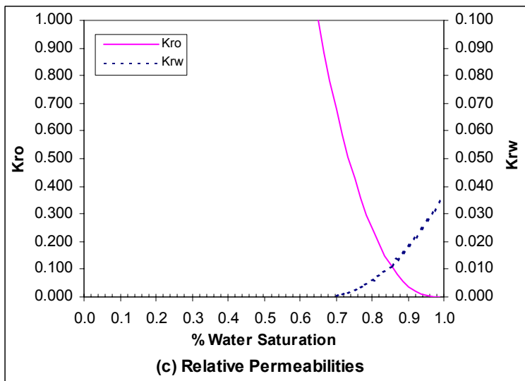
Figure A9: Coreflood Simulator Results for Waterflood of Yates Crude Oil in Berea Core with Nonionic Surfactant Concentration of 3500 ppm
