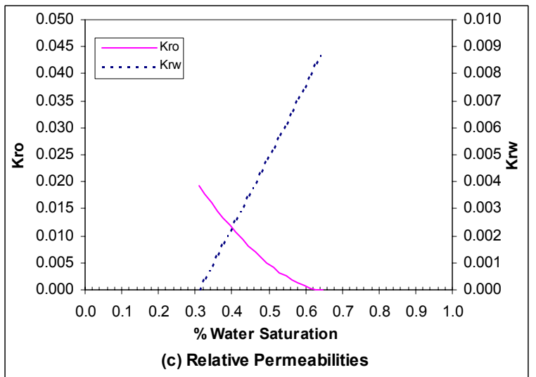
Figure A15: Coreflood Simulator Results for Waterflood of Decane in Berea Core with Anionic Surfactant Concentration of 5000 ppm
