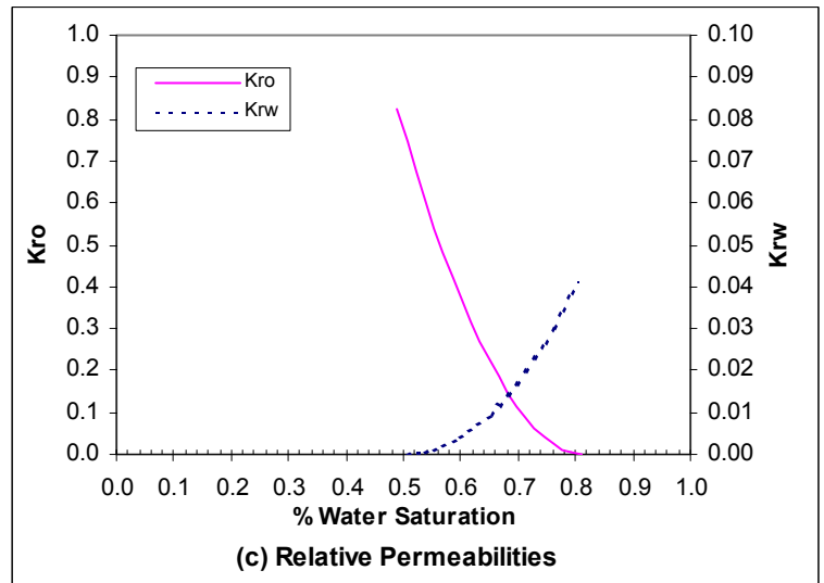
Figure A7: Coreflood Simulator Results for Waterflood of Yates Crude Oil in Berea Core with Nonionic Surfactant Concentration of 500 ppm
