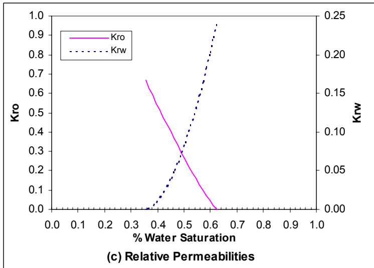
Figure A12: Coreflood Simulator Results for Waterflood of Decane in Berea Core with Anionic Surfactant Concentration of 500 ppm
