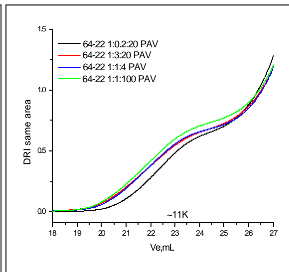
Figure 4-19 GPC traces for the AC 64-22 mixtures with redox1 (1:0.2:20), redox3 (1:1:100), redox4 (1:3:20), redox5 (1:1:4) after PAV
