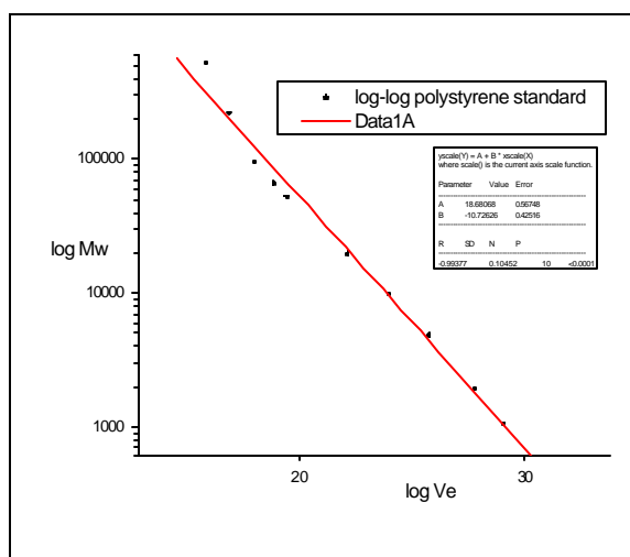
Figure 2.2.5-3 Linear calibration from PS GPC traces
