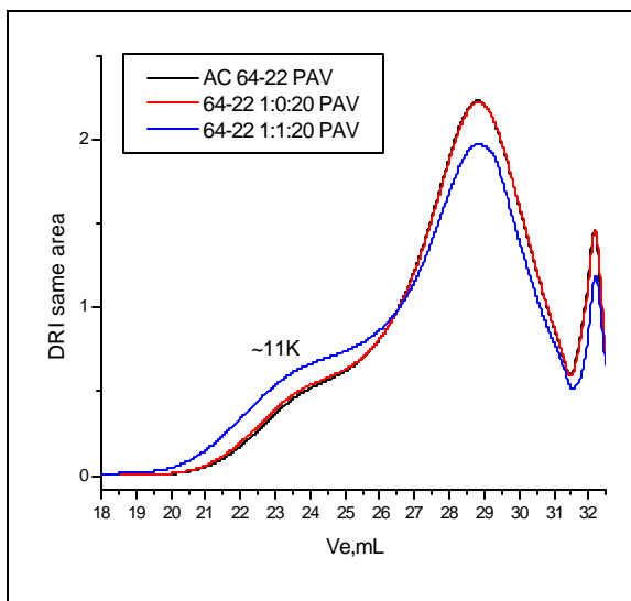
Figure 4-18 GPC traces for the AC 64-22, AC 64-22 mixtures with HP (1:0:20), redox2 (1:1:20), after dry PAV aging
