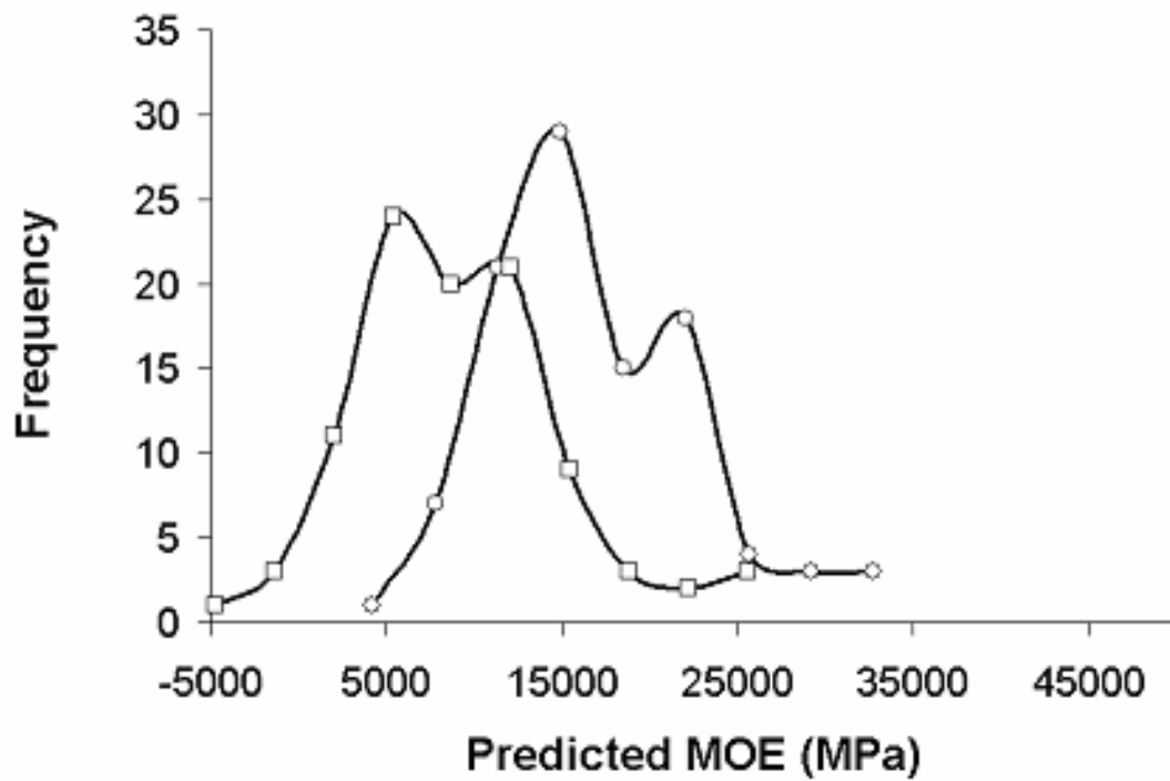
Figure 7.3: The prediction of MOE for stained (n=101) and unstained (n=101) wood using (a) PCR and (b) PCR from 1 st derivative spectra.
