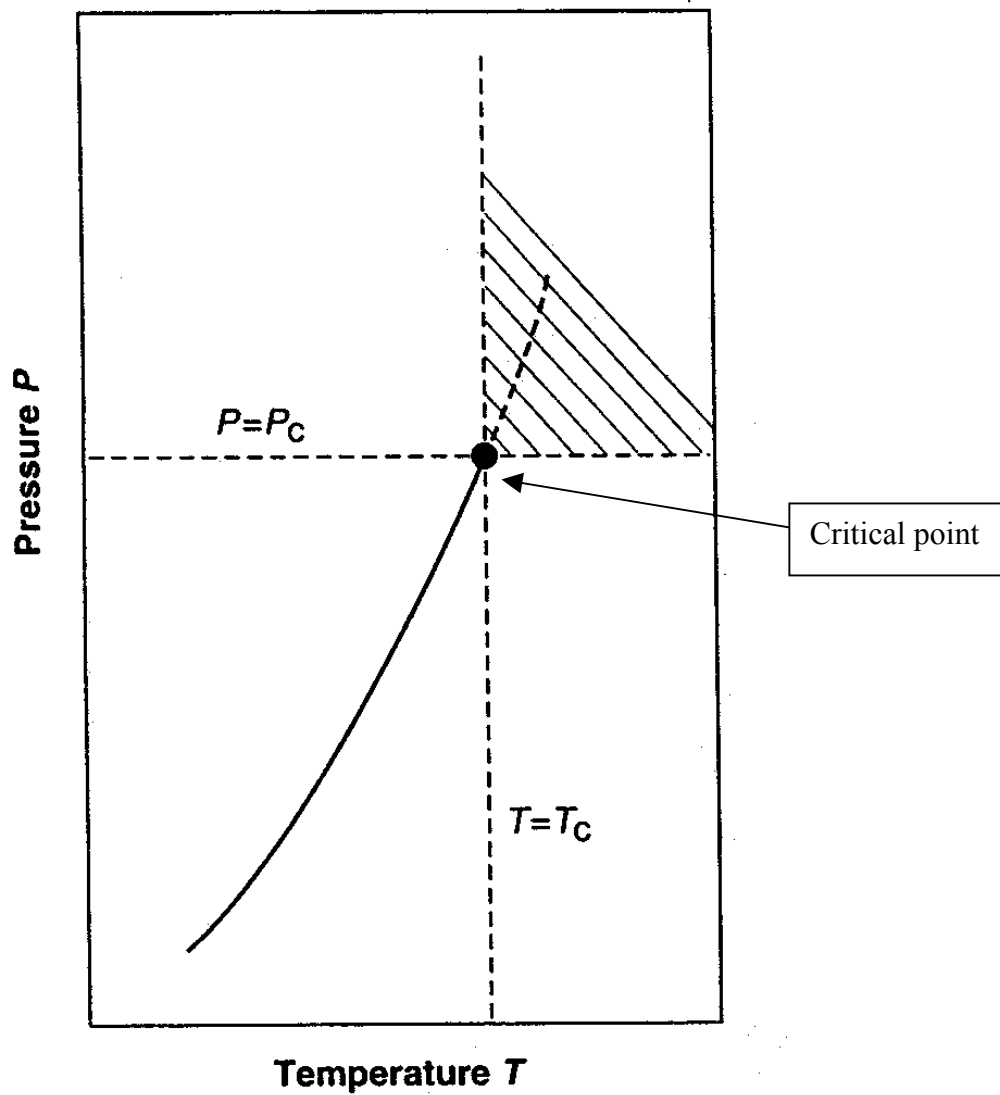
Figure 2.1. Pressure-Temperature (P-T) phase diagram of a one-component fluid (9).
