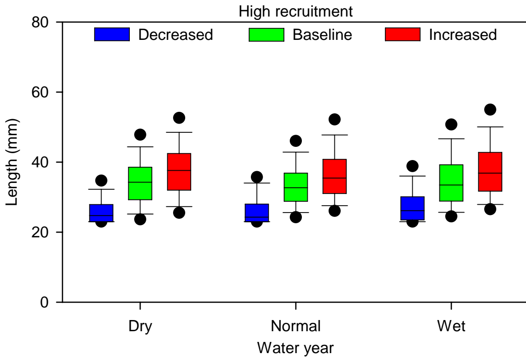
Figure 3.16 October length distributions of anchovy for dry, normal and wet years under decreased, baseline and increased nutrient loads for low and high recruitment. Circles show the 5 th and 95 th percentiles of the distributions. Whiskers show the 10 th and 90 th percentiles, the box shows the 25 th and 75 th percentiles and the solid line in the box shows the median.
