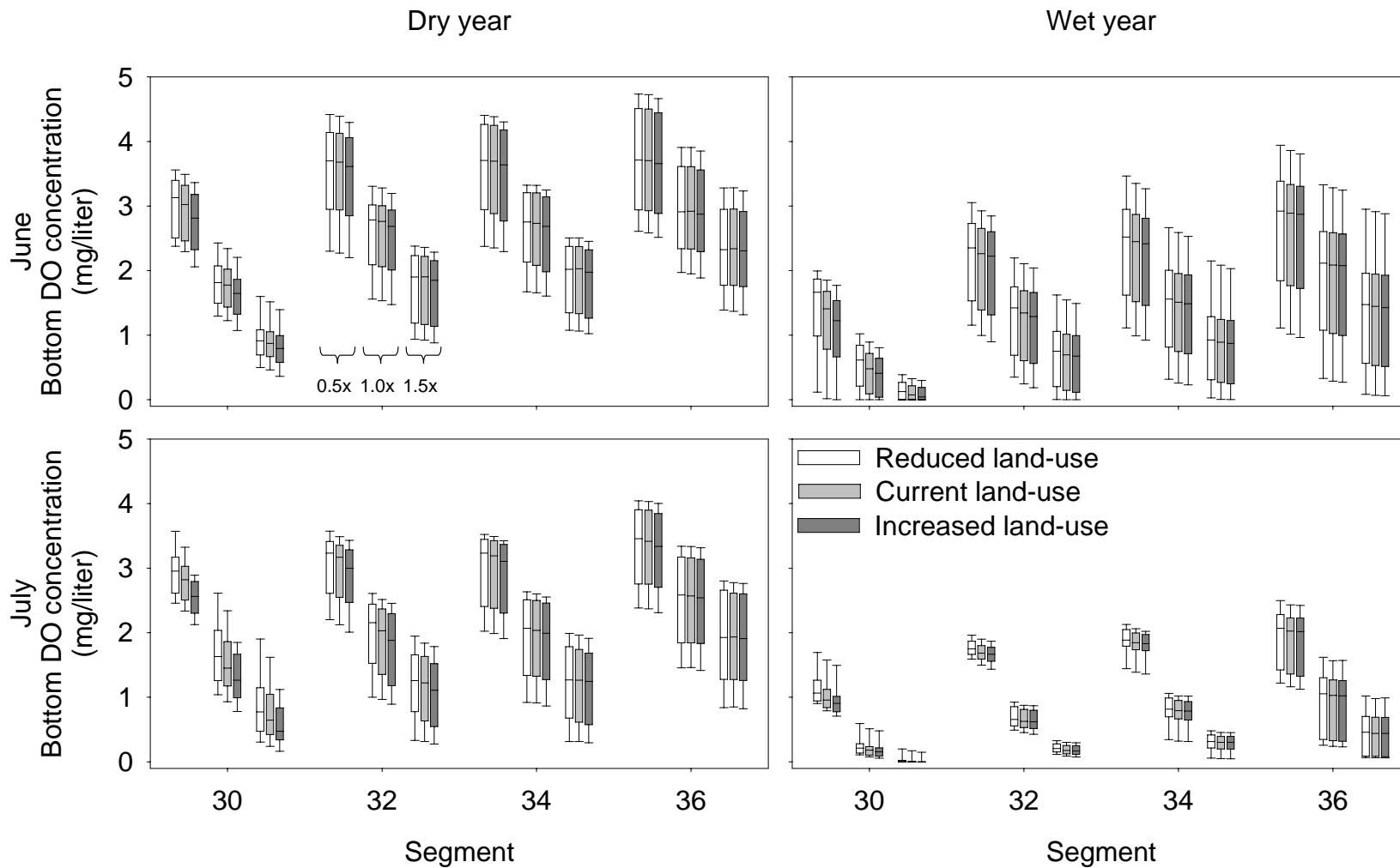
Figure 2.9 Boxplots showing monthly bottom-layer DO concentrations for wet and dry years during June and July. Whiskers show the 10 th and 90 th percentiles of the distribution. Box shows the 25 th and 75 th percentiles and the solid line in the box shows the median. Boundary condition scenarios are indicated in June-Dry year panel.
