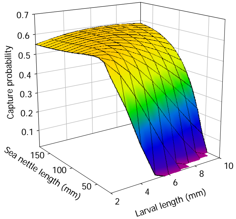
Figure 2.3 Capture probabilities of ctenophore and sea nettle predators preying upon larval bay anchovy. (A) Ctenophore (B) Sea nettle.
