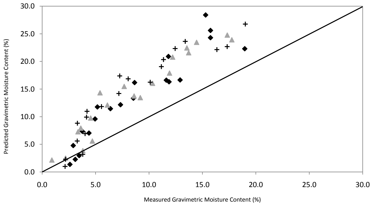
Figure 6.2: Manufacturer's generalized calibration predictions versus field measurements (% gravimetric) for Kill Devil Hill, North Carolina.
