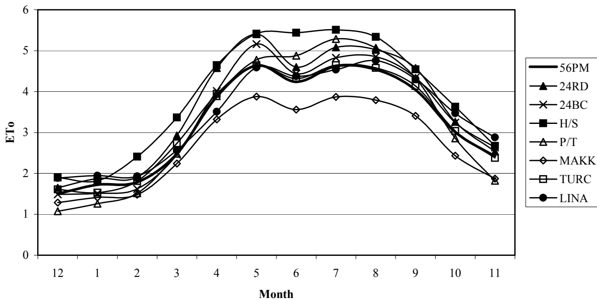
Figure 5.6 Coastal Monthly Composite ET_0 : Dec 2002 - Nov 2003
