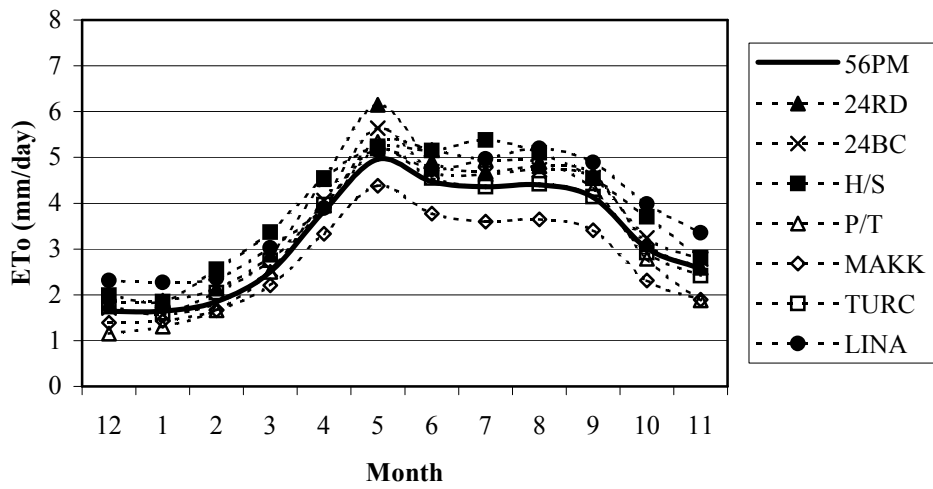
Figure 5.9 Monthly ET 0 - Houma: December 2002 - November 2003
