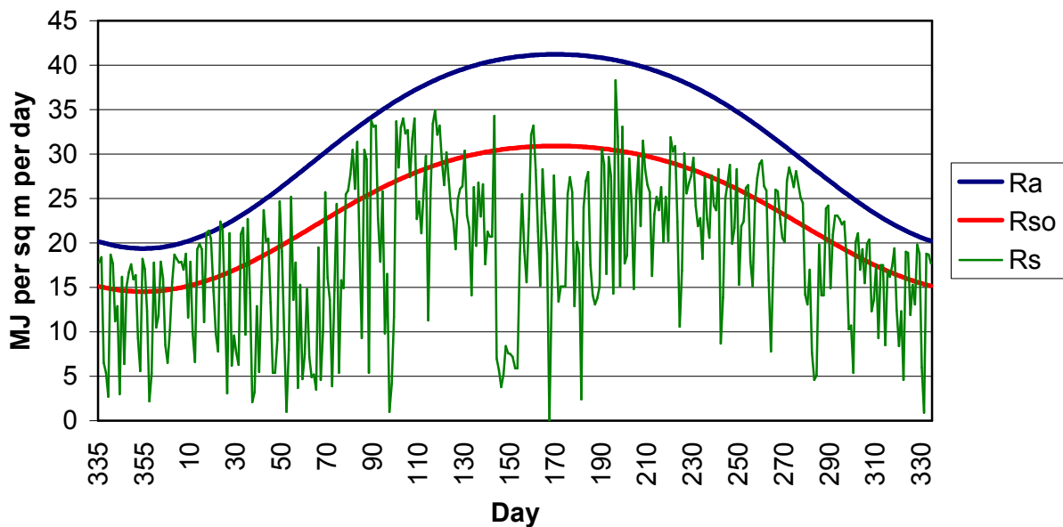
Figure 4.2 Hammond R_s values before correction. R_{s0} values are calculated using a 0.75 coefficient.
