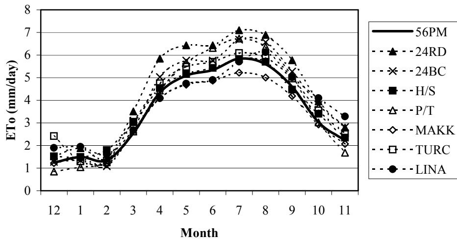
Figure 5.13 Monthly ET 0 - UL-Monroe: December 2002 - November 2003
