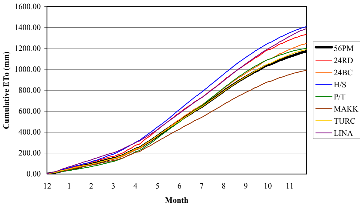
Figure 5.3 Coastal Cumulative ET 0 : December 2002 - November 2003
