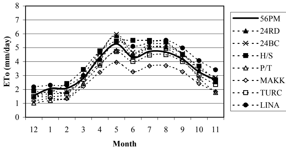
Figure 5.7 Monthly ET 0 - Ben Hur RS: December 2002 - November 2003
