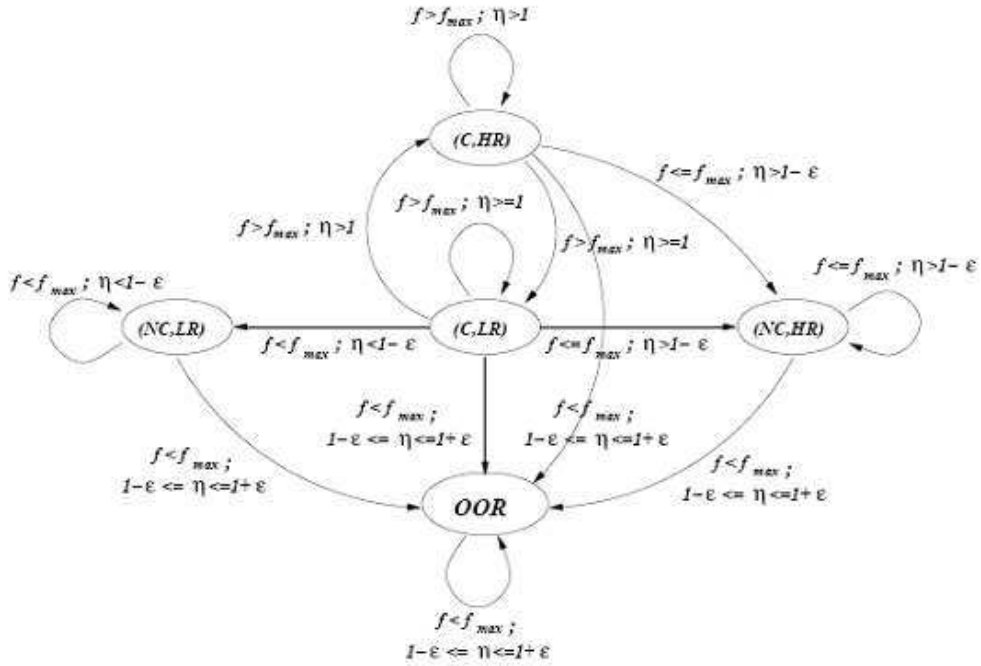
Figure 2.4: ESRT finite state machine.
