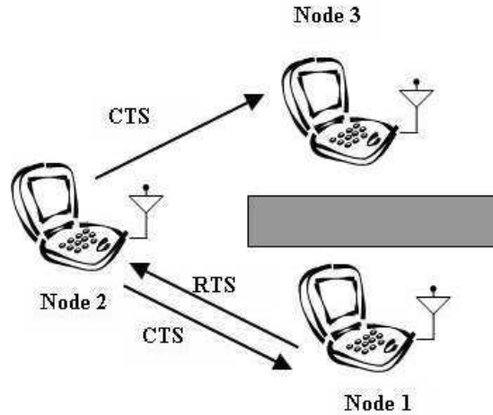
Figure 1.10: RTS-CTS messaging system.
