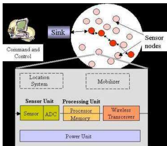
Figure 1.7: Internal structure of a sensor node.
