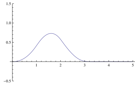
(b) \alpha = 3.6
