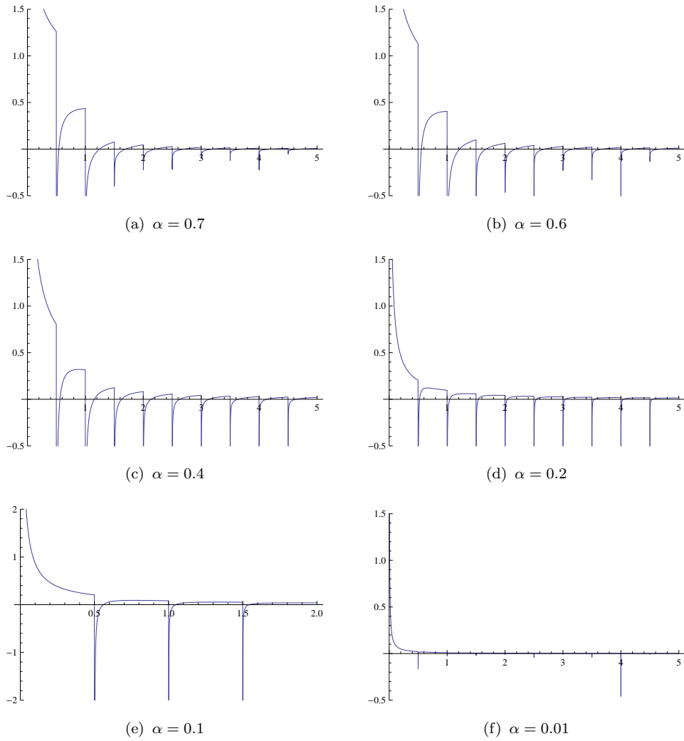
FIGURE 1.9. (a\chi_{[0,1/2]} + b\chi_{(1/2,1]})^{*\alpha}(u)
