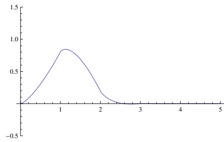
(f) \alpha = 2.8
