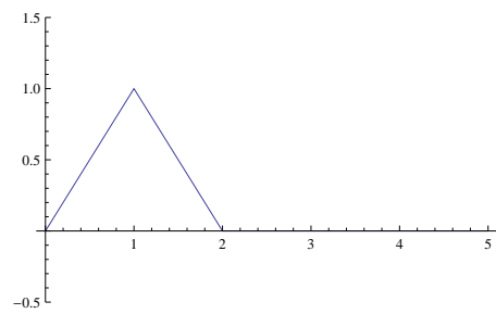
(h) \alpha = 2.0
