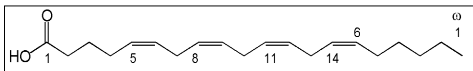
Figure 1. A schematic of the structure of arachidonic acid. Upper numbers refer to the numbering system from the methyl carbon and lower numbers refer to the number system from the acid carbon end, which is known as the delta system.
