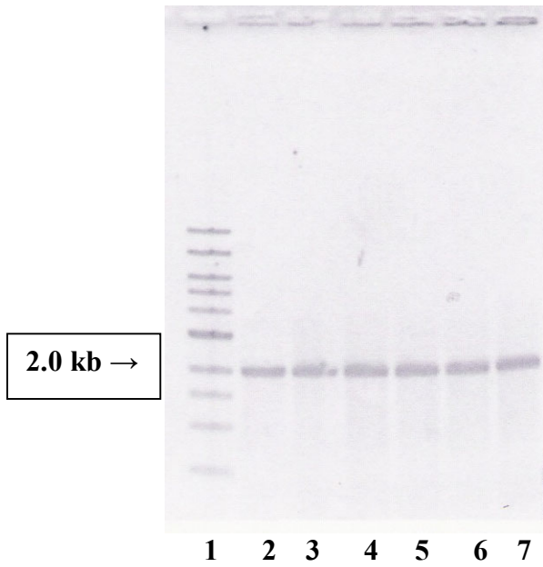
Figure 7. Agarose gel electrophoresis of PCR products amplified from pQAE miniprep DNA using the ORF-944F and ORF-944R primers. Gel reveals a ~2.0 kb Region E. The arrow indicates a 2.0 kb band on the molecular weight marker.
