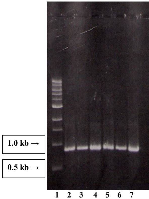
Figure 9. Agarose gel electrophoresis of an 840 bp kanamycin antibiotic cassette PCR-amplified from pBBR1MCS-2 using the KAN-AL and KAN-AR primers. The arrows indicate 0.5 and 1.0 kb bands on the molecular weight ladder.
