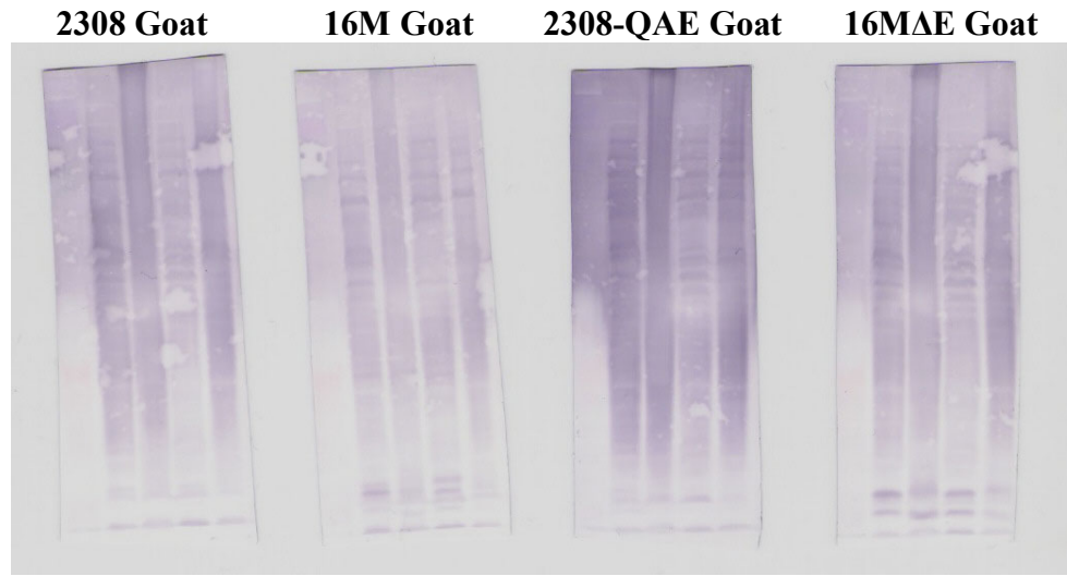
Figure 15. Western immunoblot analysis of B. abortus 2308, B. melitensis 16M, B. abortus 2308-QAE, or B. melitensis 16MΔE-infected goats. Sera were taken at necropsy, and the blots were run using cell lysates from each of the aforementioned strains.
