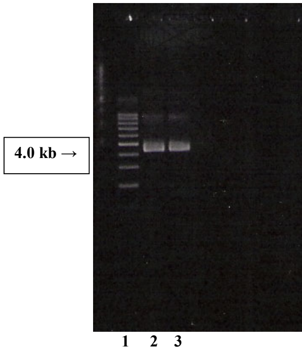
Figure 11. Agarose gel electrophoresis of pUC19 \Delta E miniprep DNA. The arrow indicates a 4.0 bp band on the molecular weight ladder.
