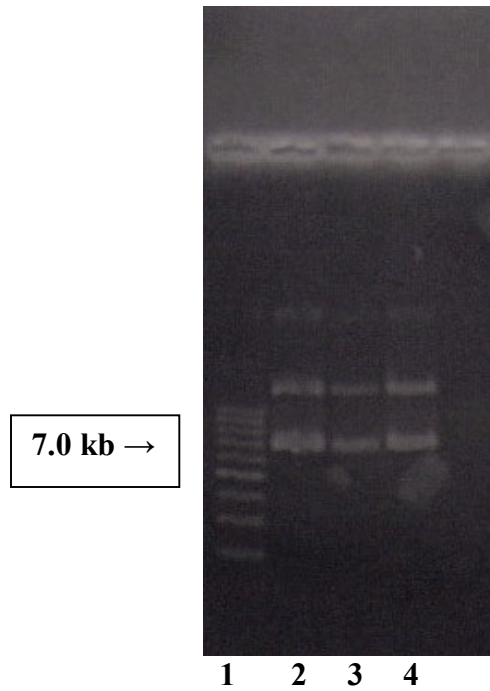
Figure 5. Agarose gel electrophoresis of pQAE following plasmid miniprep. The arrow indicates a 7.0 kb band on the molecular weight ladder.
