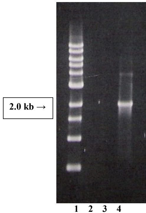
Figure 3. Agarose gel electrophoresis of the ~2.0 kilobase Region E PCR-amplified using the ORF-944F and ORF-944R primers. The arrow indicates the 2.0 kb band on the molecular weight ladder.
