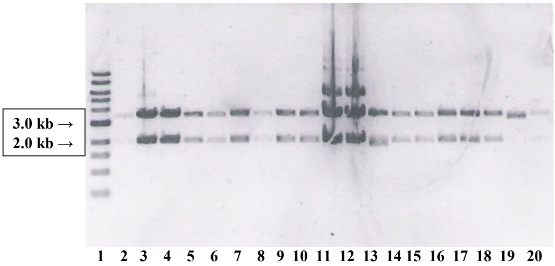
Figure 8. Agarose gel electrophoresis of the pCR ® -Blunt II-TOPO ® vector+Region E miniprep DNA digested with EcoR I. Digestion reveals a ~2.0 kb Region E fragment and a 3,519 bp linearized pCR ® -Blunt II-TOPO ® vector. The arrows indicate 2.0 and 3.0 kb bands on the molecular weight ladder.
