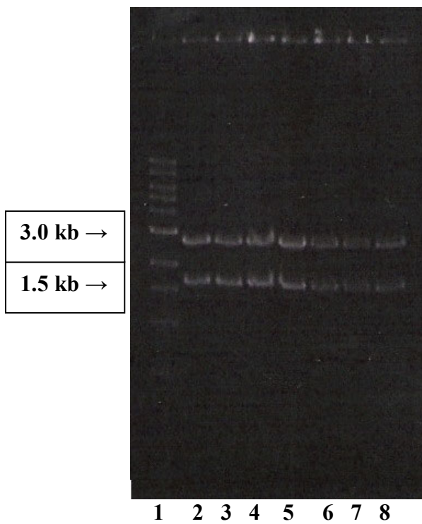
Figure 13. Agarose gel electrophoresis of pUC19ΔE digested with EcoR I. Digestion releases a 1,640 E-KAN-E fragment and linearizes a 2,678 pUC19 vector. The arrows indicate 1.5 and 3.0 kb bands on the molecular weight ladder.
