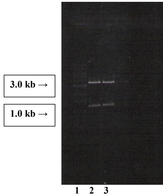
Figure 12. Agarose gel electrophoresis of pUC19ΔE digested with Age I. Digestion releases a 1,200 bp interior Region E fragment and linearizes a 3,486 bp pUC19+E vector. The arrows indicate 1.0 and 3.0 kb bands on the molecular weight ladder.
