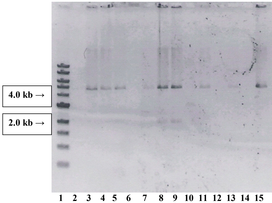
Figure 6. Agarose gel electrophoresis of pQAE miniprep DNA digested with EcoR V . Digestion reveals a ~2.0 kb Region E and a 4,950 bp linearized pBBR1MCS-4. The arrows indicate 2.0 and 4.0 kb bands on the molecular weight ladder.
