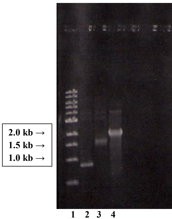
Figure 14. Agarose gel electrophoresis of PCR-amplified products from DNA isolated from B. melitensis 16M \Delta E mutants using the KAN-AL and KAN-AR and ORF-944F and ORF-944R primers. The arrows indicate 1.0, 1.5, and 2.0 kb bands on the molecular weight ladder.
