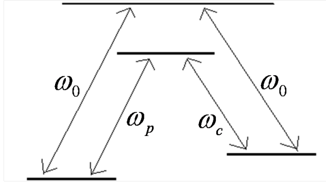
FIGURE 3.5: Schematic of a double-lambda type scheme. This will give rise to nondegenerate four-wave mixing, with photon number correlations existing between the output probe and conjugate beams. The pump beam is at frequency \omega_0 , the probe is at frequency \omega_p and the conjugate beam is at frequency \omega_c .
