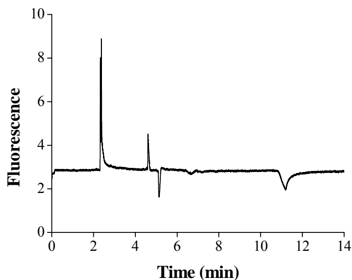
Figure 2.5. Electropherogram of an enzyme inhibition assay (inhibition of alkaline phosphatase by arsenate) using an enzyme microreactor constructed with a single magnet. Experimental conditions for loading the magnetic beads are the same as in Figure 2.2, and the same running buffer and substrate concentration were used. The inhibitor, 0.125 mM sodium arsenate, was injected for 3.0 s at 12.0 kV. Finally, a separation potential of 12.0 kV was applied.
