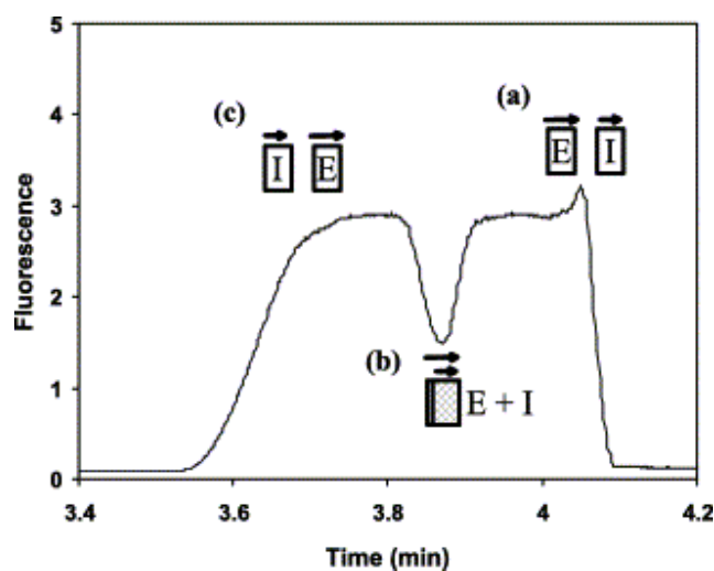
Figure 1.7. Electropherogram of a theophylline-alkaline phosphatase enzyme-inhibitor assay (Figure from Reference 51)
